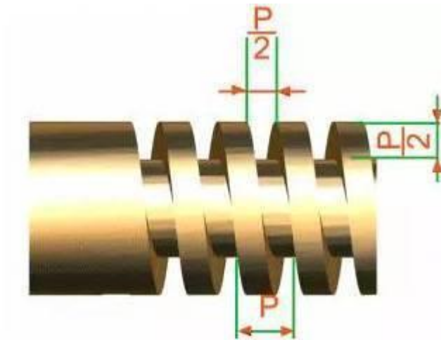
Trapezoidal Thread
