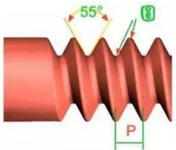
Knuckle Thread
