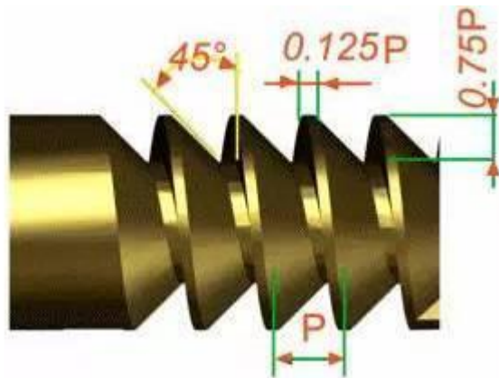
Buttress Thread
