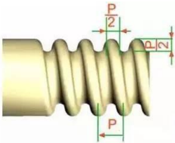
Pipe Thread
