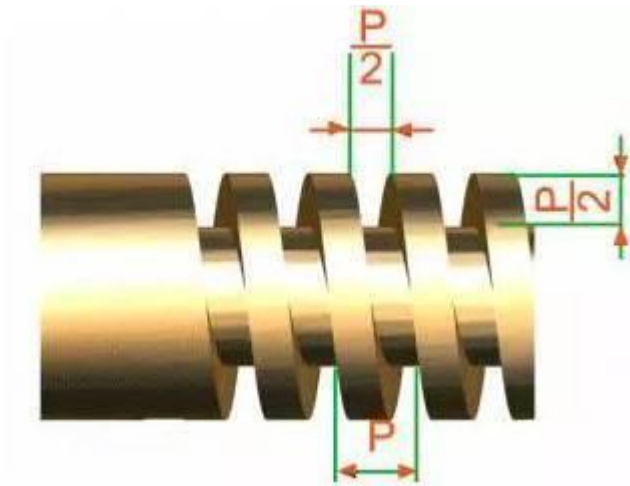
Trapezoidal Thread
