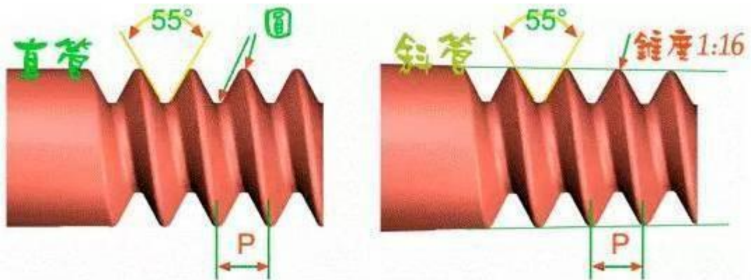
Square Thread
