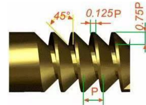
Butress Thread
