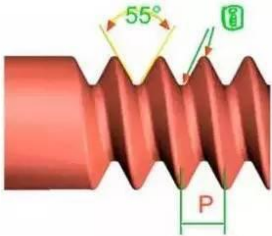
Knuckle Thread
